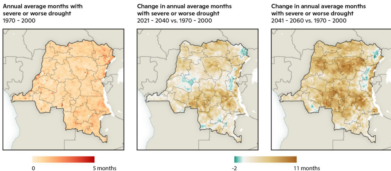
Figure 1: Change in Drought, DRC. Annual average months with severe, or worse, drought in 1970–2000 (left), and change in months in 2021–2040 (center) and 2041–2060 (right) compared to 1970–2000. Regions expected to experience additional months of drought stress are depicted in shades of brown, and regions expected to experience a decrease in months of drought stress are depicted in shades of green.
