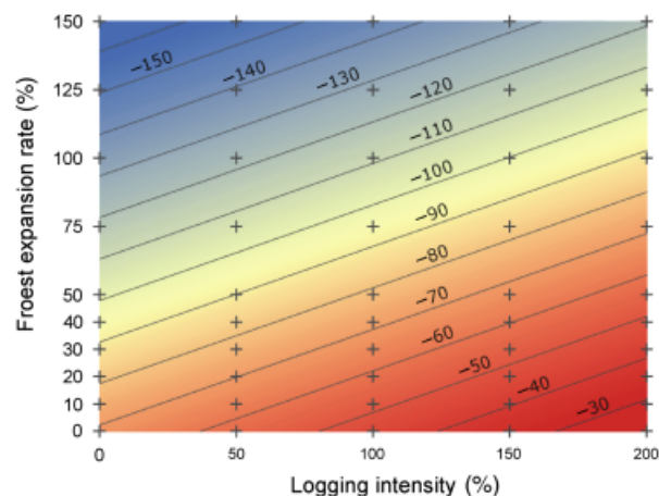
Fig. 6 Total carbon sink strength [ \text{Tg C} ] between 2008 and 2100 for different scenarios of logging intensity (100% = 5000 \text{ ha yr}^{-1} ) and forest expansion (100% = all currently unused farmland \sim 728\,000 \text{ ha} ). Crosshairs mark modeled scenarios; isolines denote identical sink strength across different scenarios.
