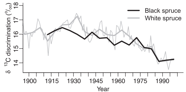
Figure 6 Stable carbon isotope ( \delta^{13}\text{C} ) time series for black spruce and white spruce stands in interior Alaska. Black spruce data were measured in the Zasada Road 8 stand at the Bonanza Creek Long-term Ecological Research (LTER) site ( 64.8^{\circ} N, 148.0^{\circ} W) following the methods described by Barber et al. (2000) and at 5-yearly intervals to assure sufficient wood material was available for analysis. Yearly white spruce \delta^{13}\text{C} discrimination (thin grey line) was taken from Barber et al. (2000), measured in the Reserve West stand in the same LTER site and averaged at 5-year intervals (bold line). Isotopic discrimination is expressed as the proportional deviation of the measured ^{13}\text{C}/^{12}\text{C} ratio from the Peedee belemnite carbonate standard (Craig 1957).
